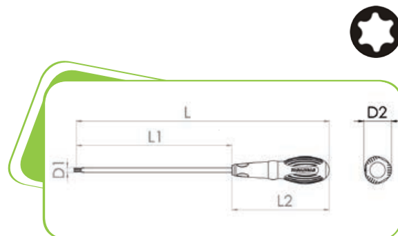
Set of extra-long screwdrivers for TX head screws
