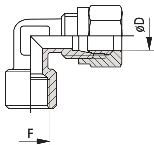
ELBOW FEMALE ADAPTOR
