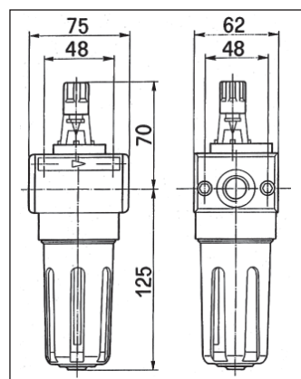
L60 TM OIL-MIST LUBRICATOR
