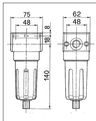
F60 TM STEAM SEPARATOR FILTER
