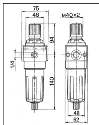
FR60 TM PRESSURE FILTER-REGULATOR
