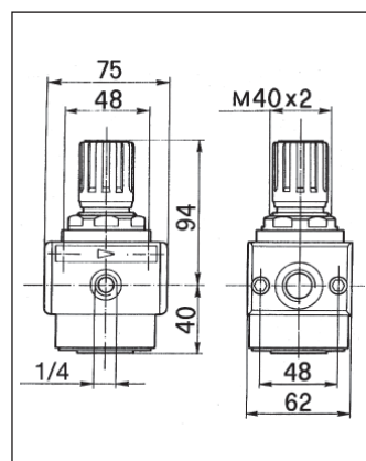
R60 PRESSURE REGULATOR
