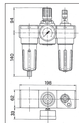
FRL 60 THREE-UNIT COMPLETE GROUP
